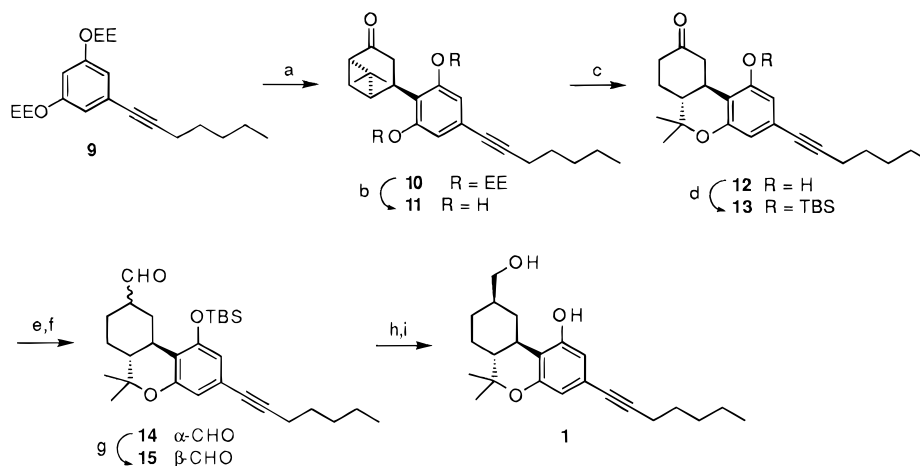
Scheme 2. Synthesis of 3-Hept-1-ynyl-11-hydroxyhexahydrocannabinol a
